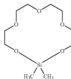
dimethylsila-14-crown-5; and
