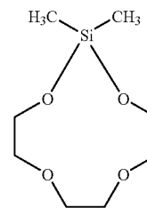
dimethylsila-11-crown-4;
